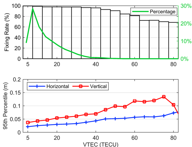
Fig. 11 Variation in RTK positioning results during years of low solar activity with respect to VTEC. The top panel represents the fixing rate, with green line indicating the percentage of VTEC in each interval. The bottom panel illustrates the 95% confidence level for horizontal and vertical accuracy
