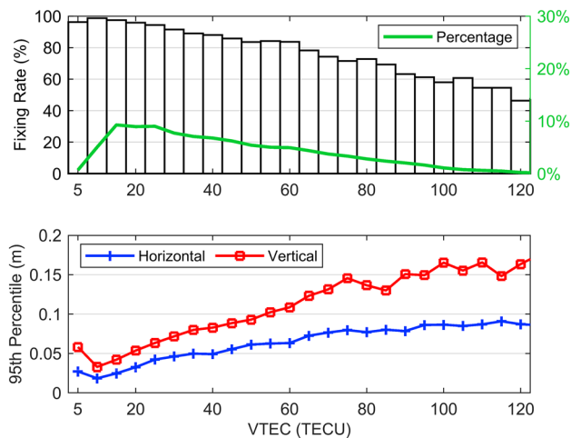
Fig. 10 Variation in RTK positioning results during years of high solar activity with respect to VTEC. The top panel represents the fixing rate, with green line indicating the percentage of VTEC in each interval. The bottom panel illustrates the 95% confidence level for horizontal and vertical accuracy
